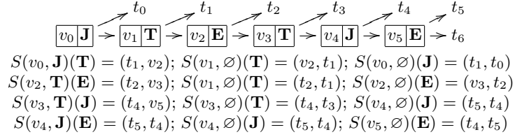
Fig. 11. The formalization of Winning a fortune , consisting of \text{ExAc}(\mathbf{J}, \mathbf{T}) , \text{UnEv}(\mathbf{T}) , \text{UnAc}(\mathbf{T}, \mathbf{J}) , and \text{UnEv}(\mathbf{J}) .
