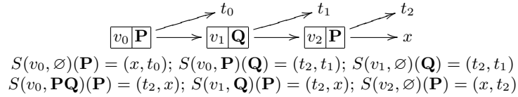
Fig. 5. The basic building block \text{Betr}(\mathbf{P}, \mathbf{Q}) of Betrayal .
